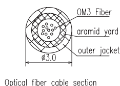
Optical fiber cable section
